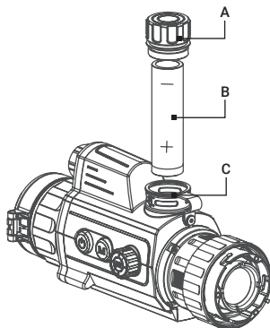
FIGURE 2-1. BATTERY INSTALLATION
