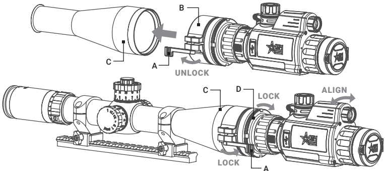
FIGURE 2-6. CLIP-ON INSTALLATION
