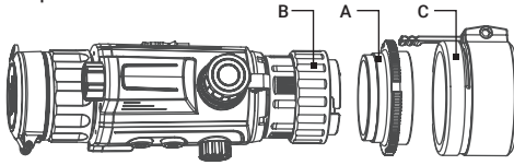
FIGURE 2-5. FRONT Q-R ADAPTER INSTALLATION
